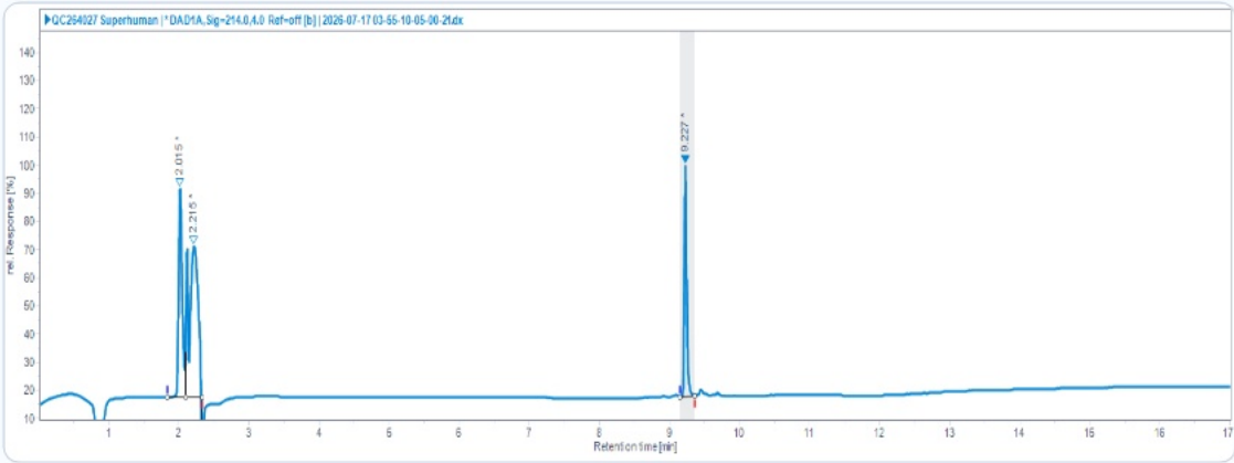
HPLC Chromatogram (Retention Time: 2.015, 2.215, 9.227 min)
